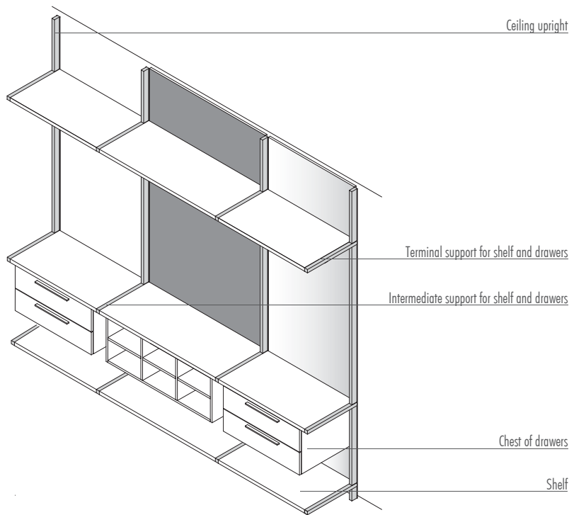
COMPONENTS' LIST OF CEILING SOLUTION
