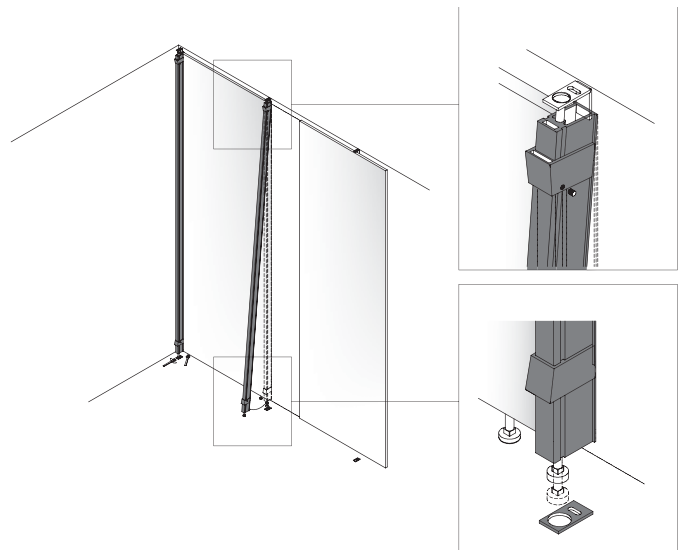
ASSEMBLING SEQUENCE
