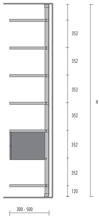
CENTRE TO CENTRE DISTANCE EQUIPMENT POSITION
