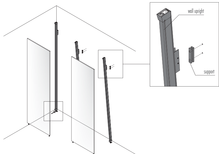
ASSEMBLING SEQUENCE
