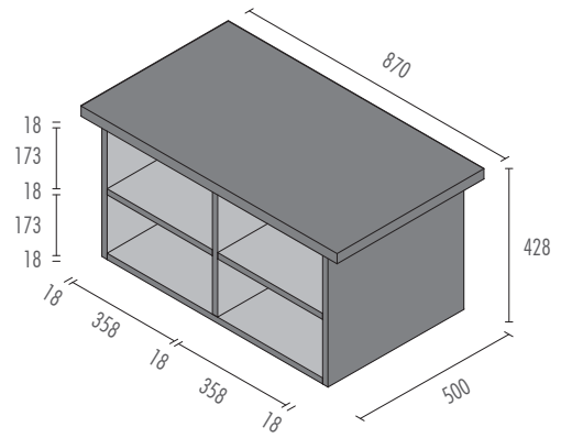
Open base unit for W 1200 module
