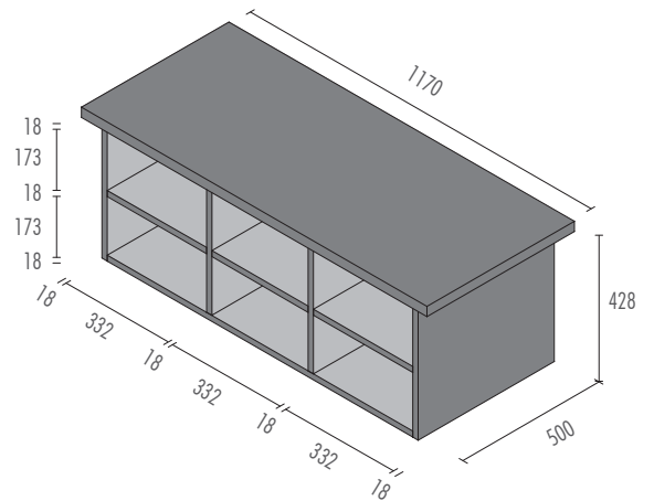
Open base unit for W 1200 module
