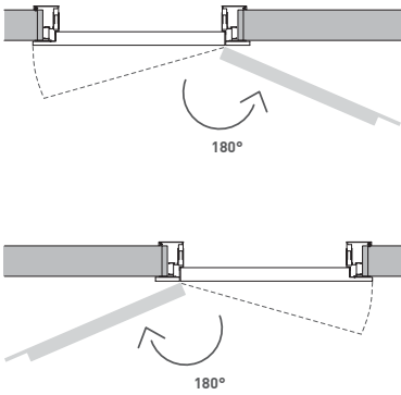
Pianta | Plan | Plan | Plan | Planta
