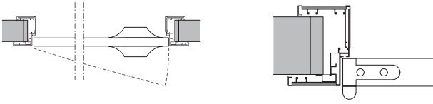
Coprifili personalizzabili | Customized finishing lists | Montants personnalisés | wahlweisen Verkleidungen | Tapetas personalizables
